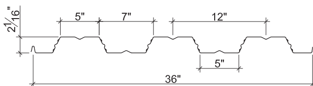
PLW2-36 or W2-36 FormLok
